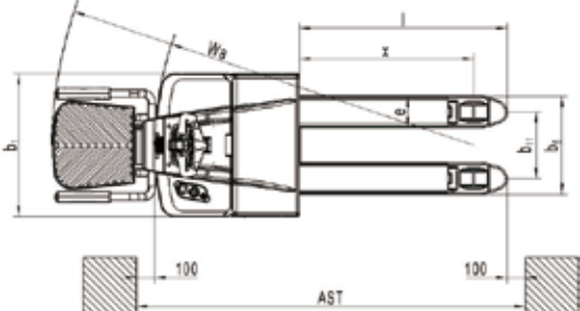
PT 20/25P-C Foldable
